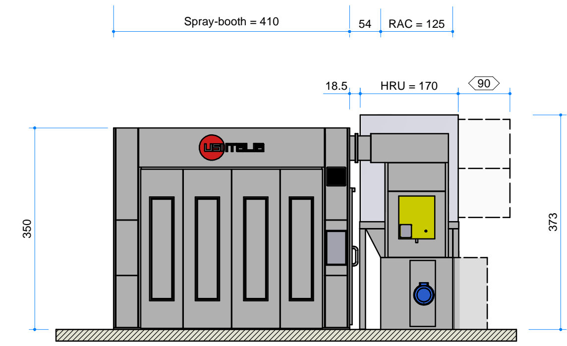
Front view Spray-booth = 410 54 RAC = 125 60
